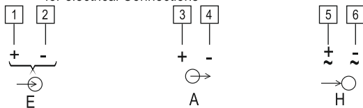
Fig. 6. Front View of Device for electrical Connections
